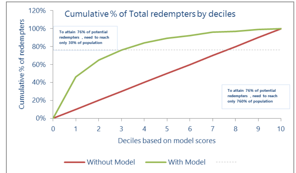
Lift Chart
